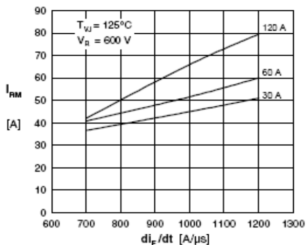
Fig. 23. Typ. peak reverse current I_{RM} vs. di/dt
