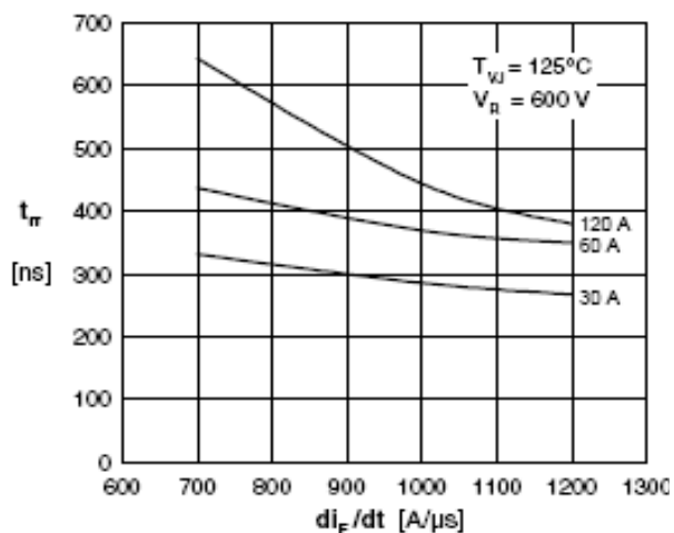
Fig. 24. Typ. recovery time t_{tr} versus di/dt
