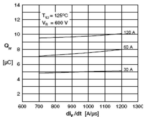
Fig. 22. Typ. reverse recov.charge Q_{rr} vs. di/dt
