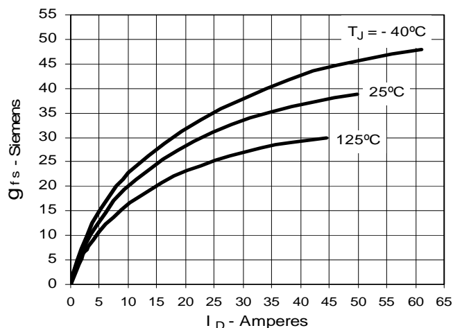
Fig. 8. Transconductance
