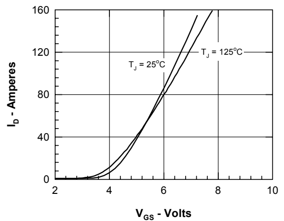
Figure 6. Admittance Curves
