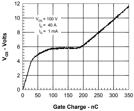
Figure 7. Gate Charge
