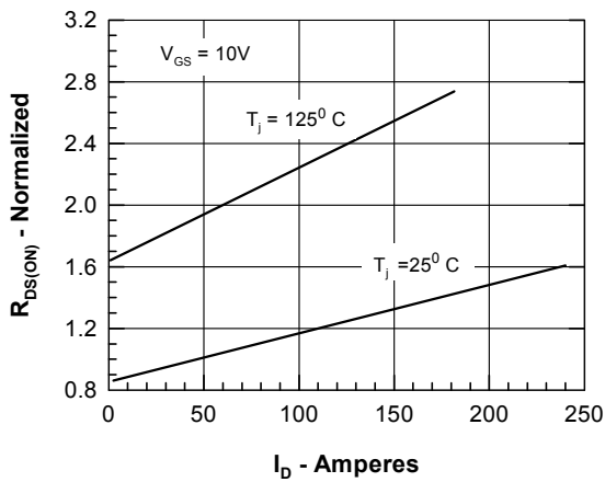
Figure 3. R_{DS(on)} normalized to 0.5 I_{D25} value
