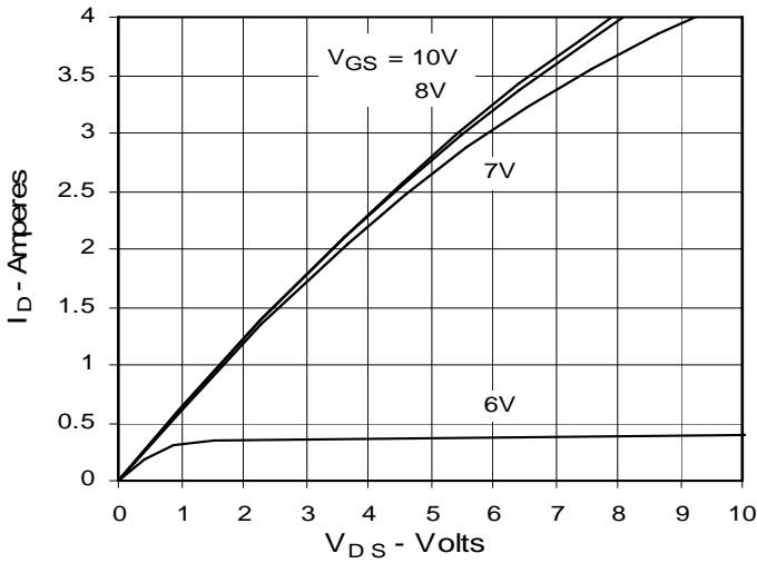
Fig. 1. Output Characteristics @ 25°C
