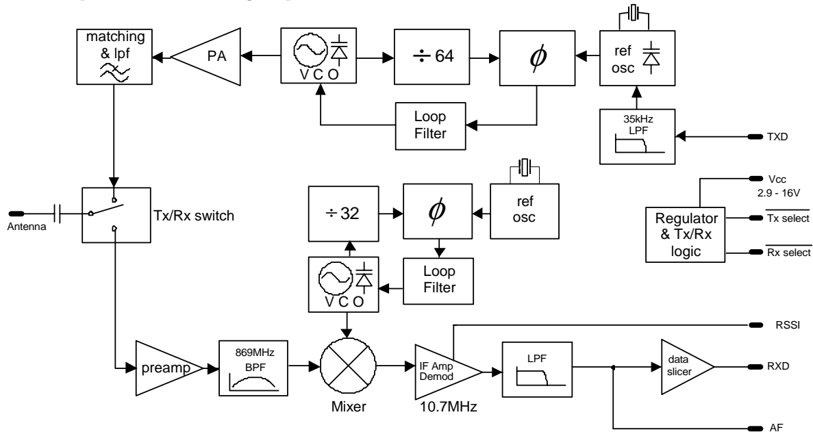
Fig. 2: Block diagram
