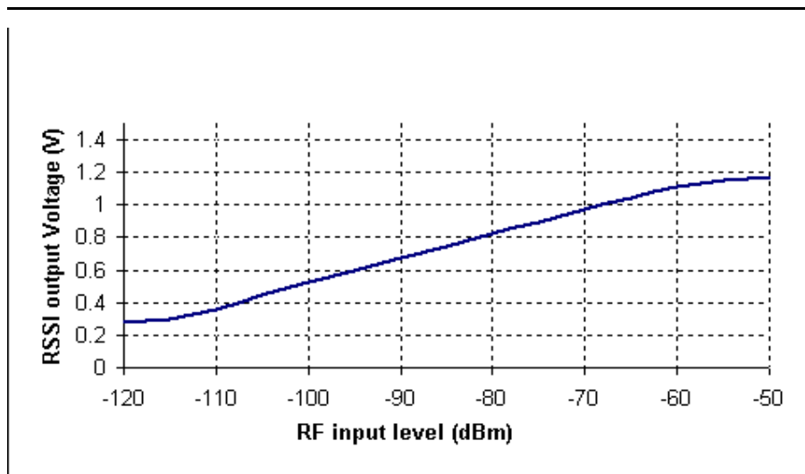
Fig.4: Typical RSSI response curve
