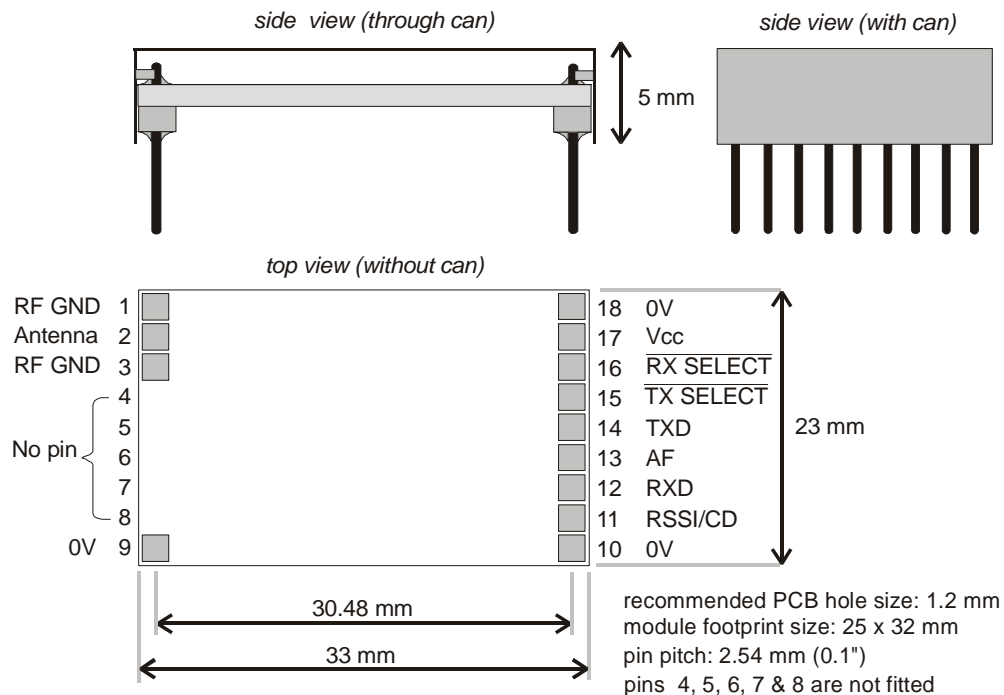
Fig. 3: Physical dimensions
