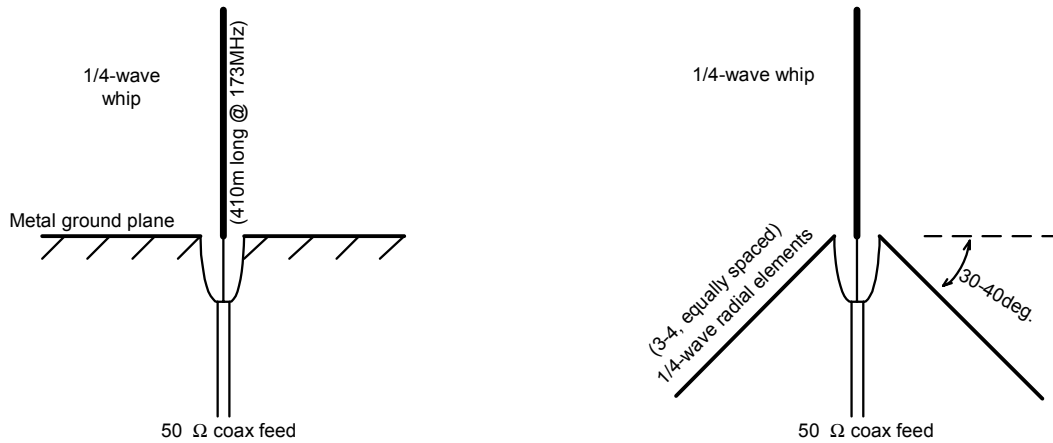
Figure 6: Quarter wave antenna / ground plane configurations
