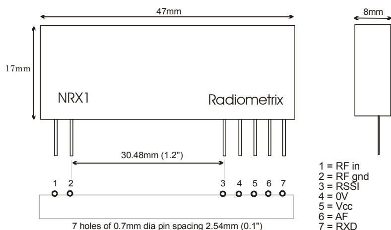
Figure 3: NRX1 pin-out and dimension
