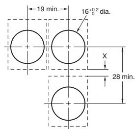
Panel Cutout (Top View)
