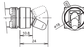
Solder/Tab Terminal
