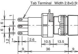
Solder/Tab Terminal
