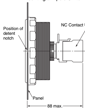
Mounting a 1-pole Switch Unit *
