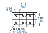
PC board pattern (Bottom view)
