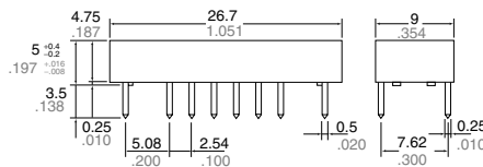
Standard PC board terminal
