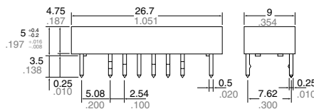
Self-clinching terminal
