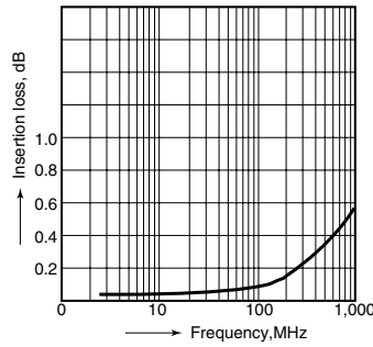
11.-(2) High-frequency characteristics Insertion loss characteristics
