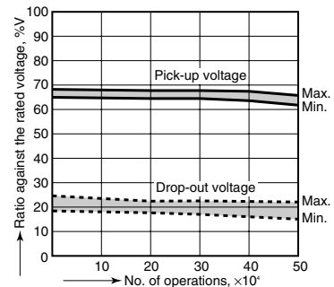
Change of pick-up and drop-out voltage
