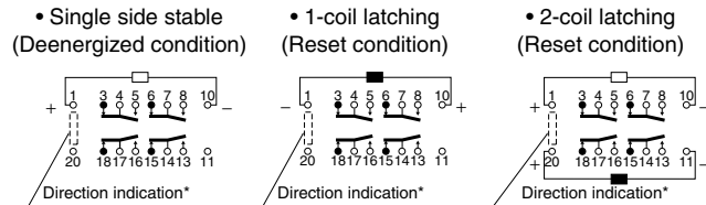
Schematic (Bottom view)
