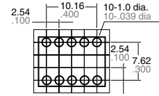
PC board pattern (Copper-side view)
