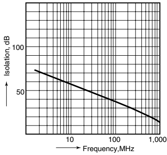
11.-(1) High-frequency characteristics Isolation characteristics
