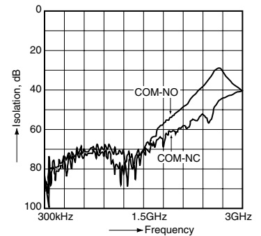
• Isolation characteristics
