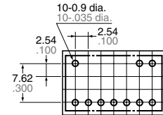
2 coil latching
