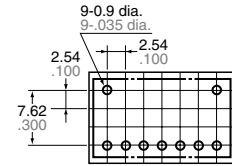
Single side stable and 1 coil latching
