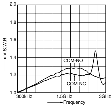
• V.S.W.R. characteristics
