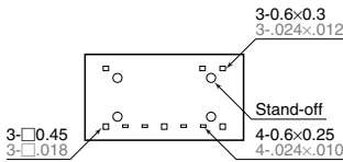
2 coil latching
