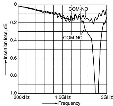
• Insertion loss characteristics
