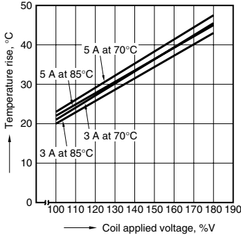
4-(1). Ambient temperature characteristics (1 Form A type)
