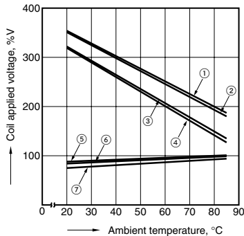
Tested sample: JQ1a-24V-F Contact carrying current: 3 A, 5 A
