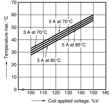
4-(2). Ambient temperature characteristics (1 Form C type)
