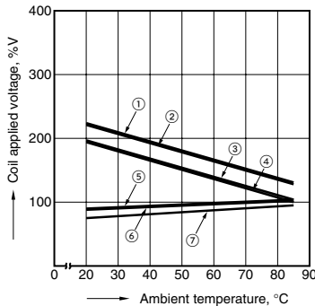
Tested sample: JQ1-24V-F Contact carrying current: 3 A, 5 A
