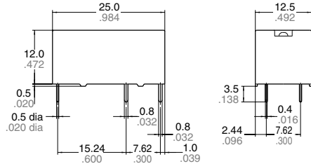
Single side stable 1 coil latching type
