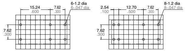
PC board pattern (Bottom view) Single side stable 1 coil latching type 2 coil latching type
