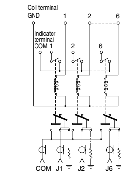
Fail-safe type
