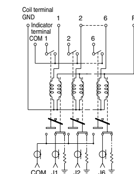
Latching type
