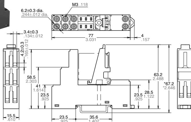
External dimensions
