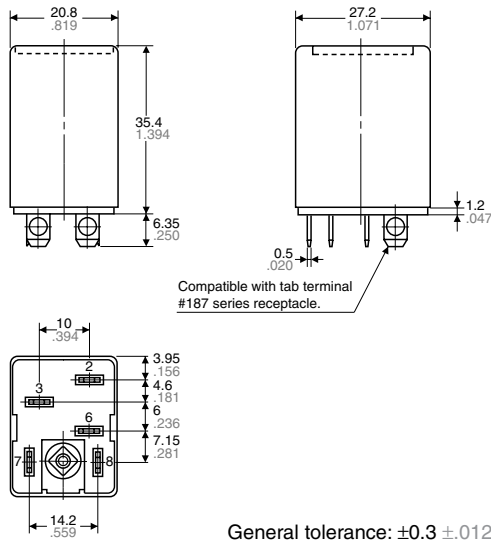
External dimensions
