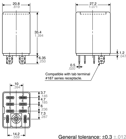
External dimensions
