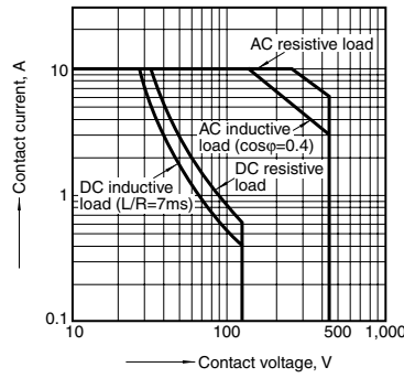
Switching capacity range (2 Form C)
