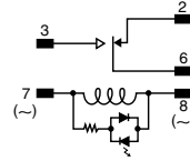
LED AC type
