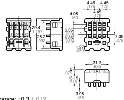
External dimensions
