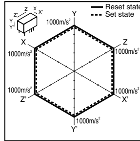
9-(2). Malfunctional shock (latching) Tested sample: TXS2-L2-4.5V, 6 pcs.
