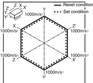
12.-(2) Malfunctional shock (latching) Tested sample: TQ2SA-L2-12V, 6 pcs.
