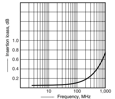
11.-(2) High-frequency characteristics Insertion loss characteristics
