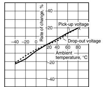
9. Ambient temperature characteristics Tested sample: TQ2SA-12V, 5 pcs.
