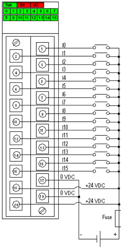
Positive Logic Wiring
