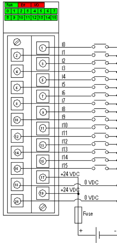
Negative Logic Wiring
