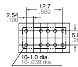
PC board pattern (Bottom view)
