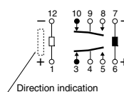
2 coil latching (LT)
