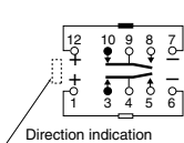
2 coil latching (L2)
