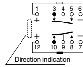
Schematic (Bottom view) 2 coil latching (L2)
