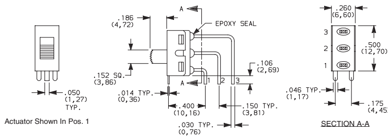
1101M2S3AV2BE2 Vertical Actuation SPDT
