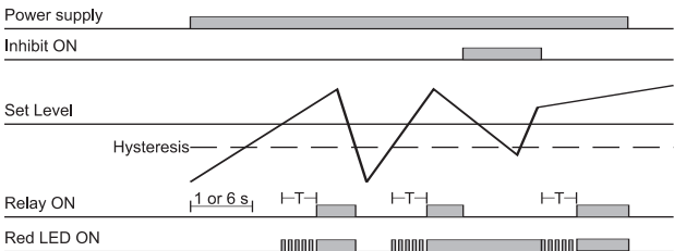
Over voltage - Inhibit function - N.D. relay
