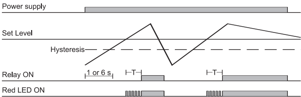
Over voltage - N.D. relay
