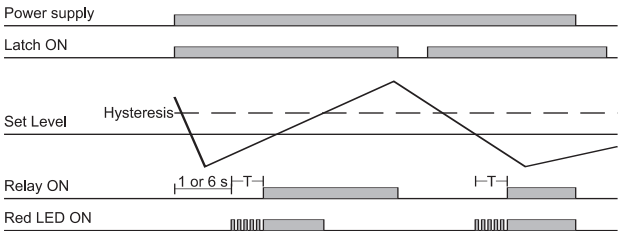
Under voltage - Latch function - N.D. relay
