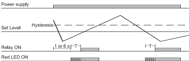
Under voltage - N.D. relay
