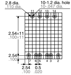
PC board pattern
