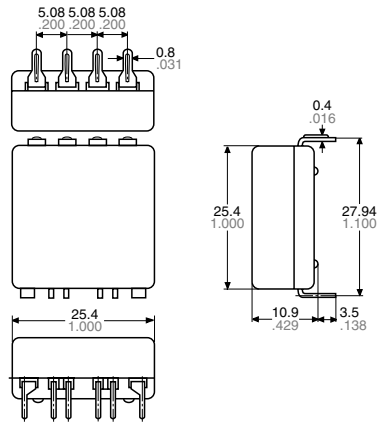
External dimensions
