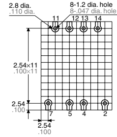
2 coil latching
