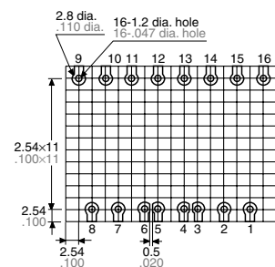
2 coil latching
