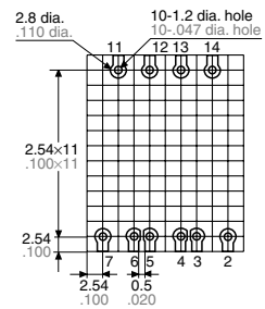
2 coil latching
