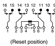
2 coil latching
