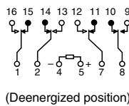
Schematic (Top view) Single side stable
