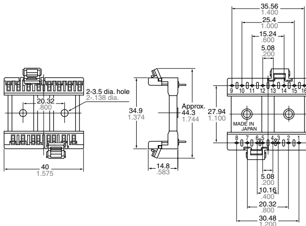
External dimensions
