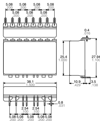
External dimensions
