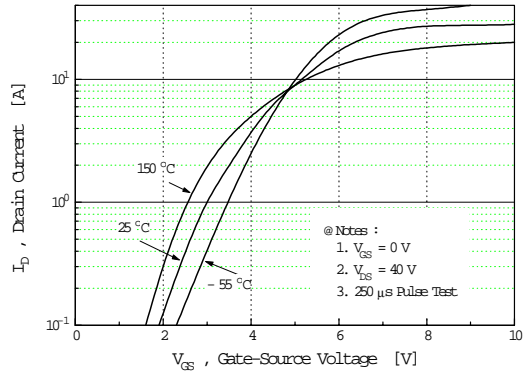
Fig 2. Transfer Characteristics
