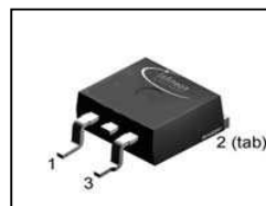
P-TO263-3-2
