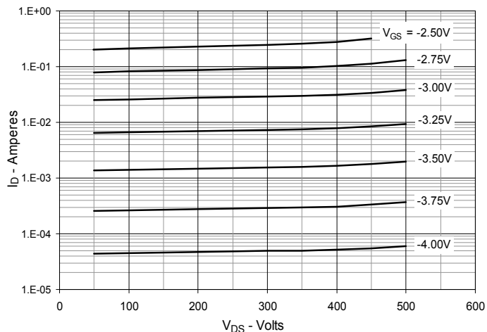
Fig. 5. Drain Current @ T_J = 100^\circ\text{C}
