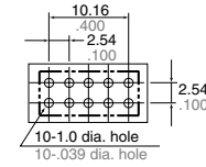
PC board pattern (Copper-side view)
