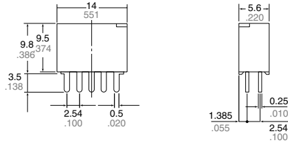
Self-clinching terminal
