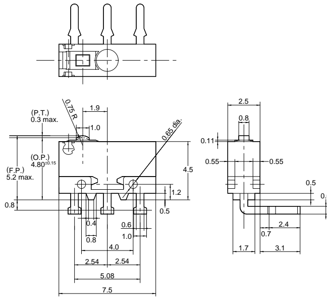
Right angle terminal
