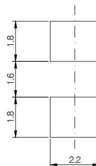
Recommended Solder Pattern
