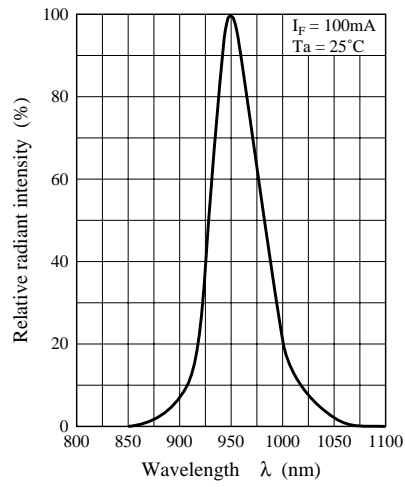
Spectral characteristics
