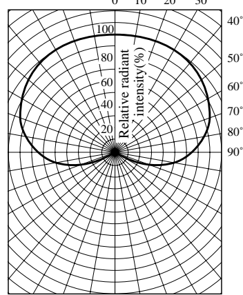
Directivity characteristics
