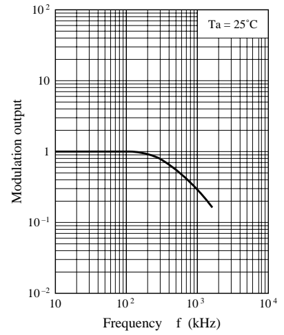
Frequency characteristics
