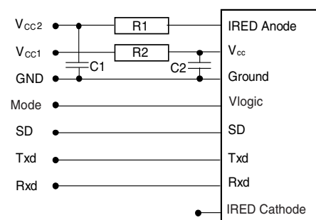
Figure 1. Recommended Application Circuit
