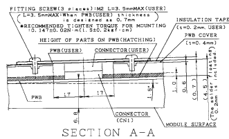
Fig 1. OUTLINE DIMENSIONS (LQ104S1DG61)
