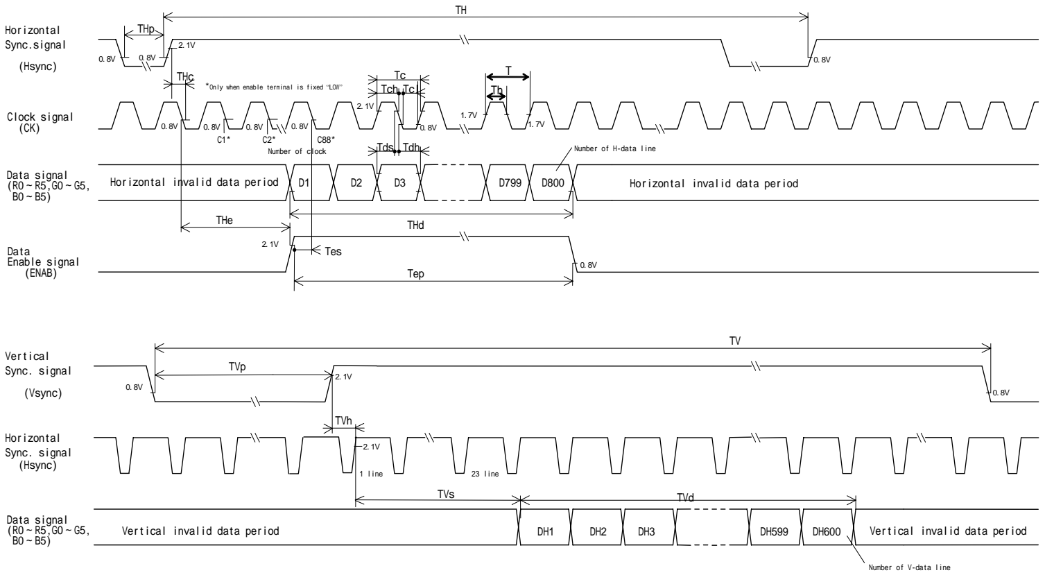
Fig. 2 Input signal waveforms
