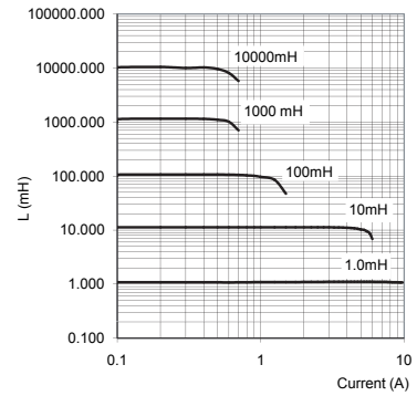
Typical L s vs Current (I)
