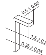
Detail of a lead
