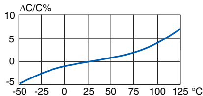
Typical capacitance vs temperature at 1 kHz
