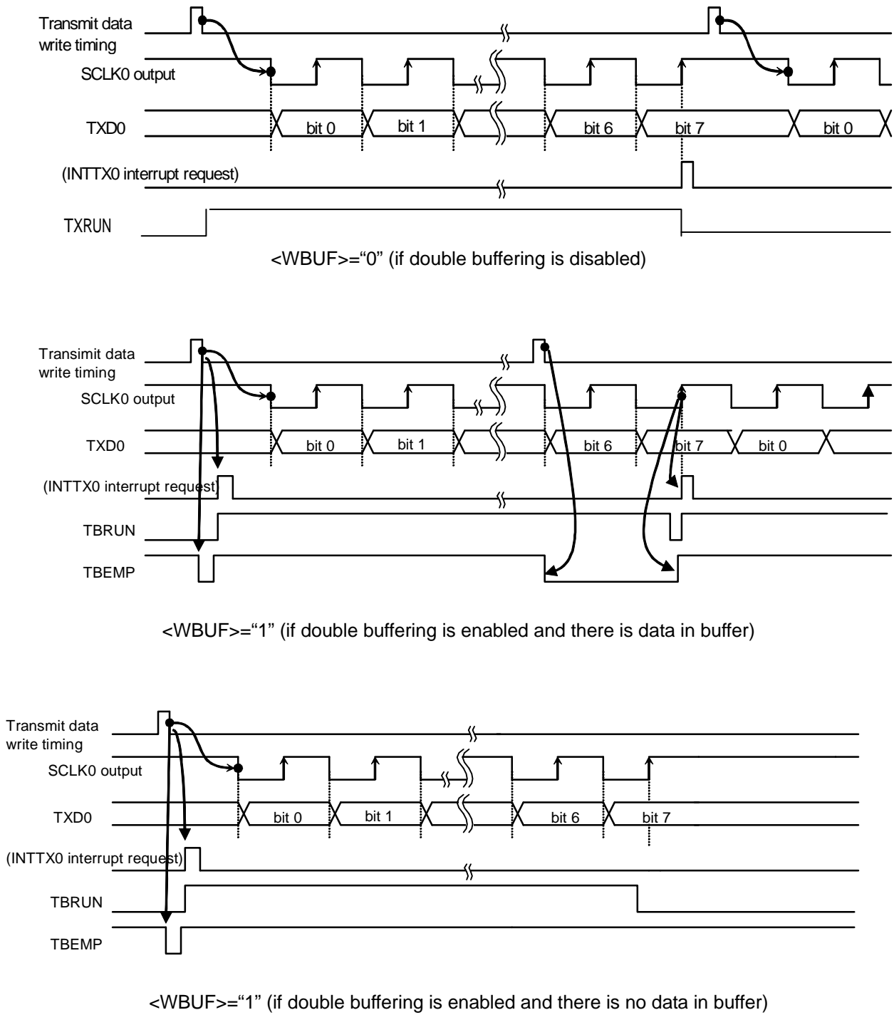
Fig 13-10 Transmit Operation in the I/O Interface Mode (SCLK0 Output Mode)
