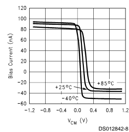
Inverting Input, Bias Current vs Common Mode Voltage V_S = \pm 1.1\text{V}
