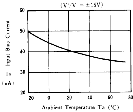
Input Bias Current vs. Ambient
