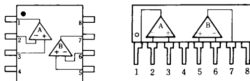
NJM4558L NJM4559L
