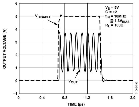
Figure 35. AD8063 \overline{\text{DISABLE}} Function, Voltage = 0 V to 5 V
