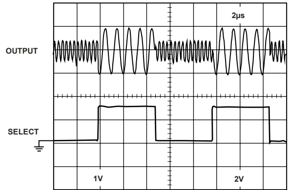
Figure 57. AD8063 Mux Output
