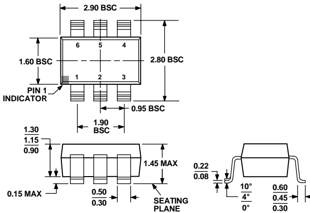
Figure 60. 6-Lead Small Outline Transistor Package [SOT-23] (RJ-6)
