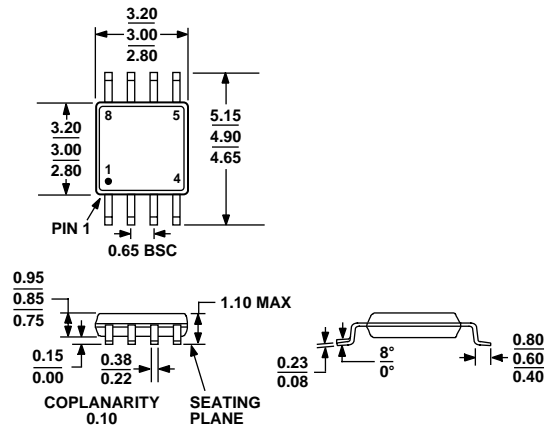
Figure 61. 8-Lead Mini Small Outline Package [MSOP] (RM-8)
