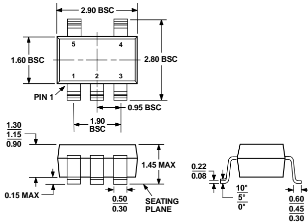
Figure 58. 5-Lead Small Outline Transistor Package [SOT-23] (RJ-5)
