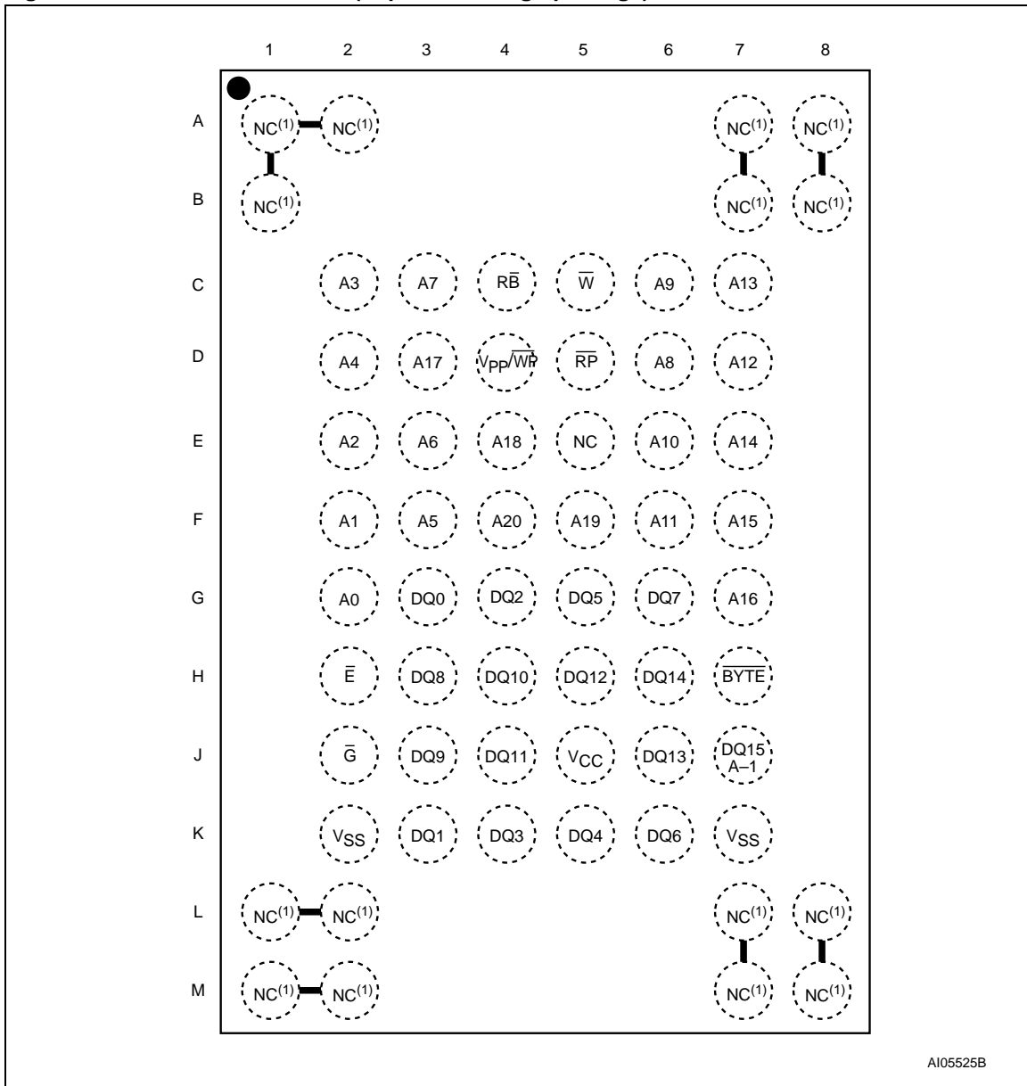
Figure 4. TFBGA63 Connections (Top view through package)
