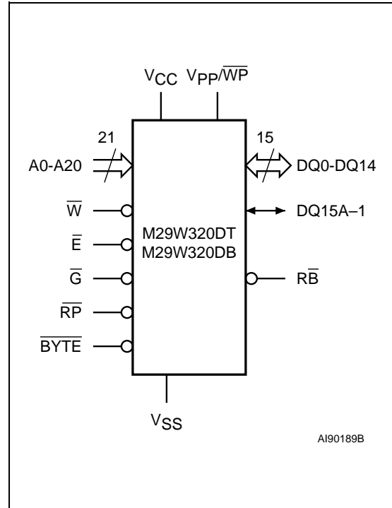
Figure 2. Logic Diagram
