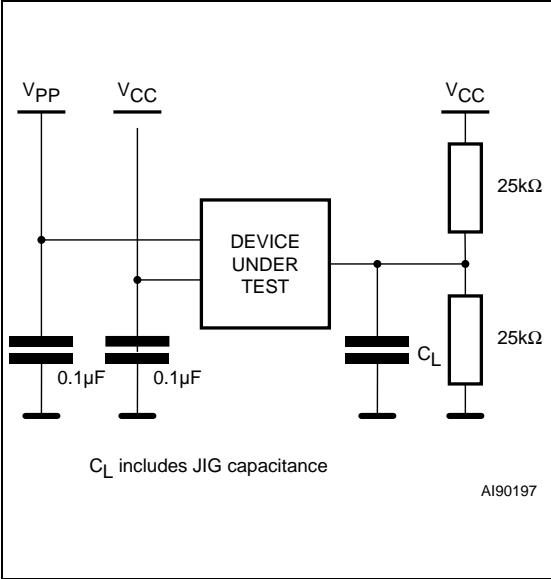
Figure 12. AC Measurement Load Circuit
