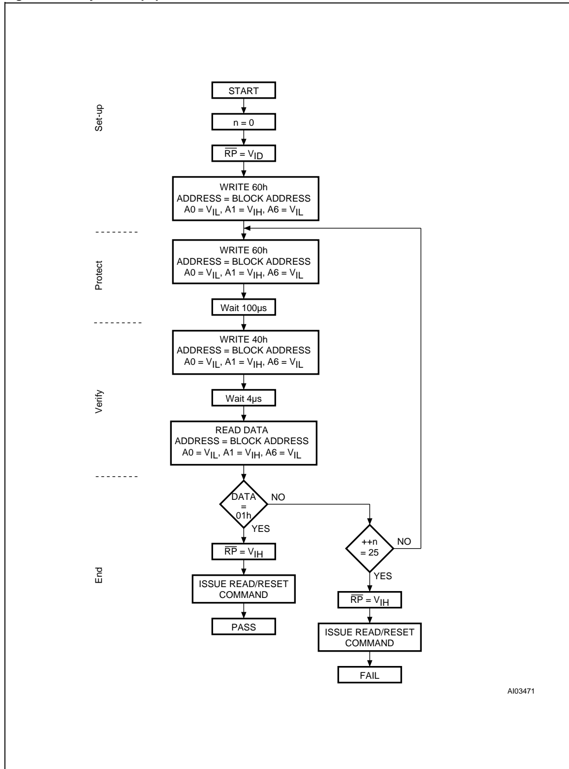
Figure 23. In-System Equipment Block Protect Flowchart
