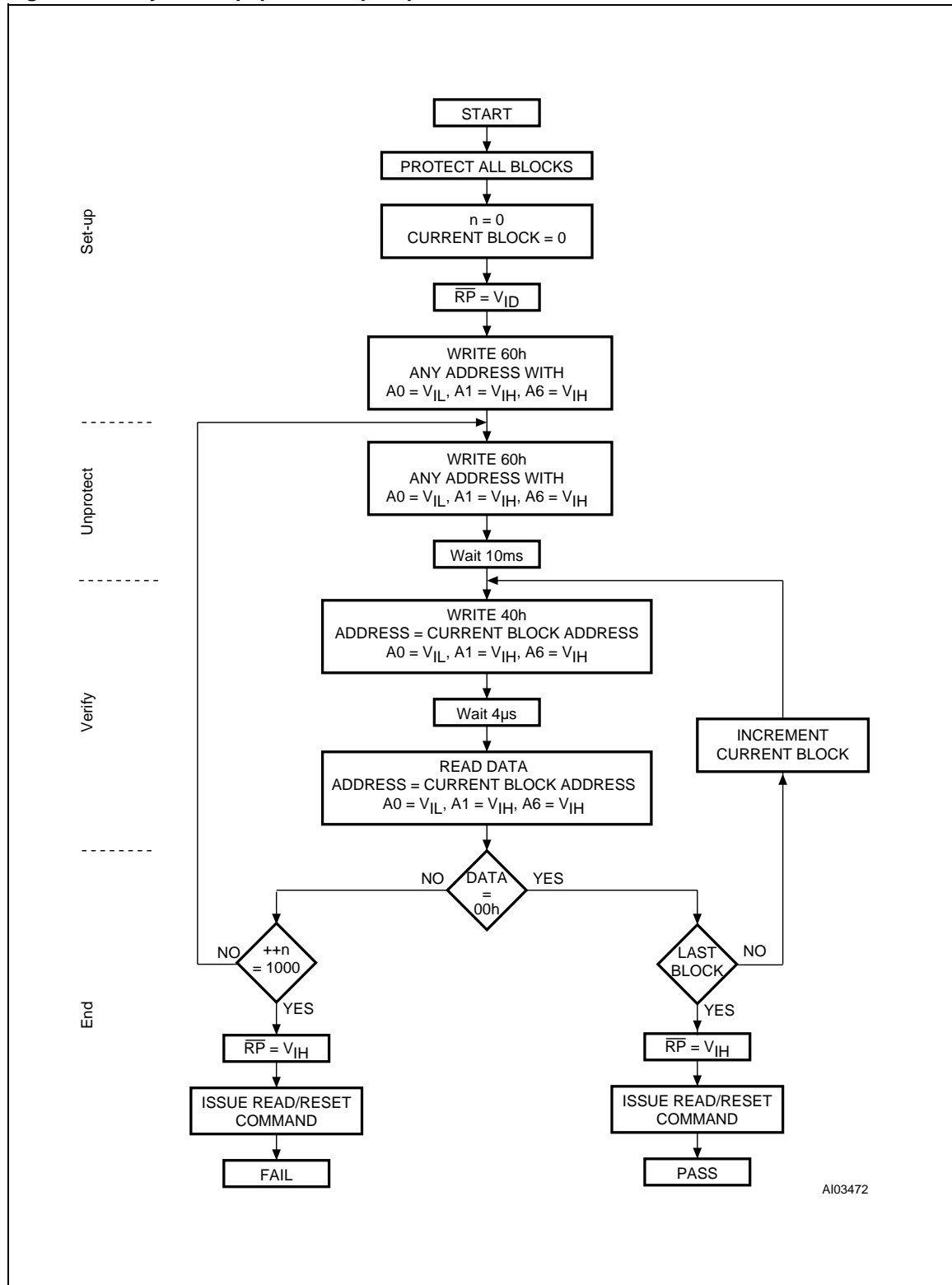
Figure 24. In-System Equipment Chip Unprotect Flowchart
