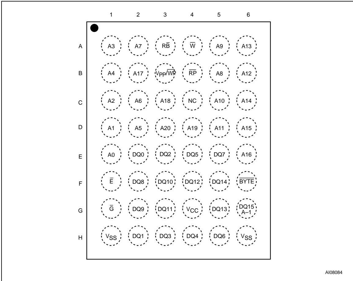
Figure 5. TFBGA48 Connections (Top view through package)
