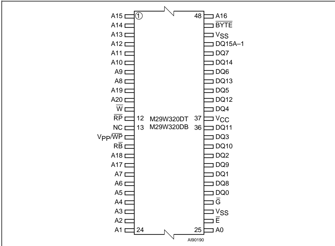
Figure 3. TSOP Connections
