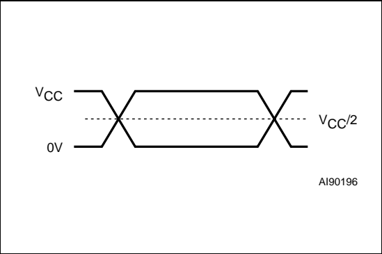
Figure 11. AC Measurement I/O Waveform
