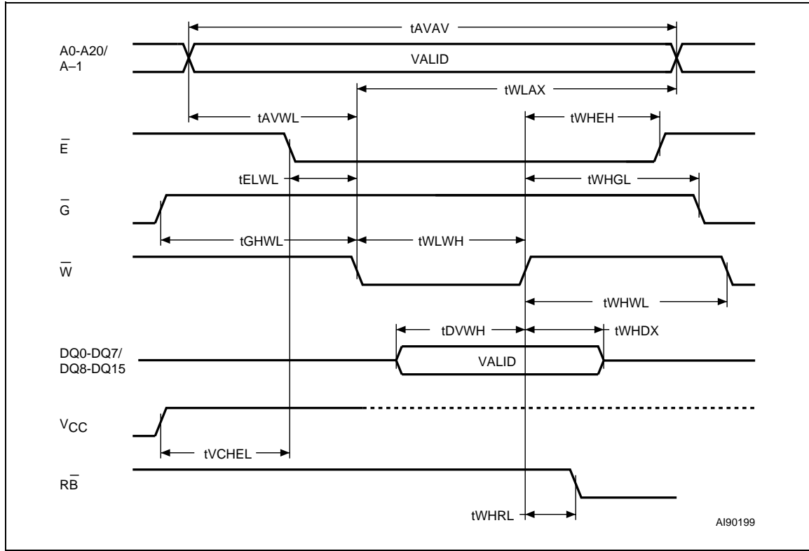
Figure 14. Write AC Waveforms, Write Enable Controlled
