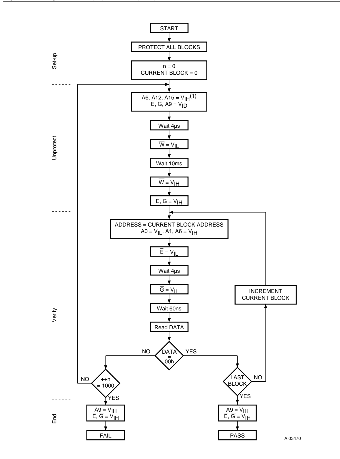
Figure 22. Programmer Equipment Chip Unprotect Flowchart
