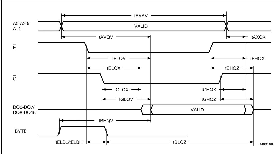
Figure 13. Read Mode AC Waveforms
