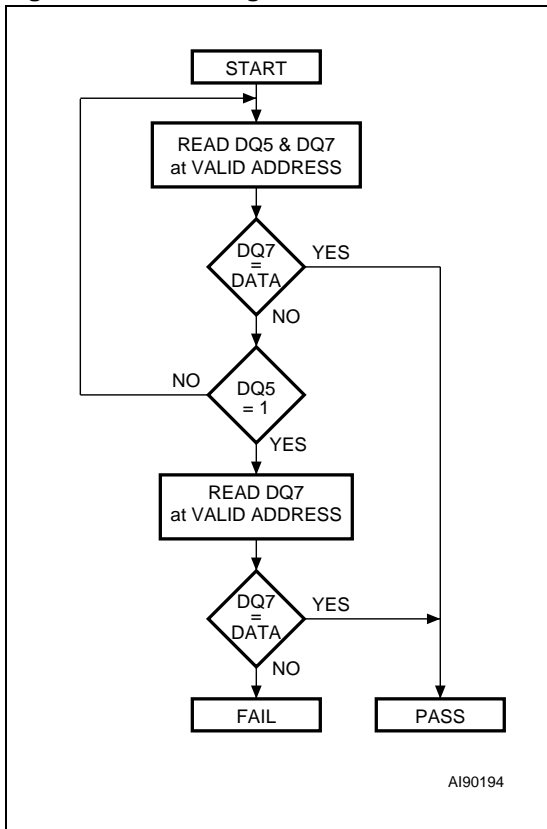
Figure 9. Data Polling Flowchart
