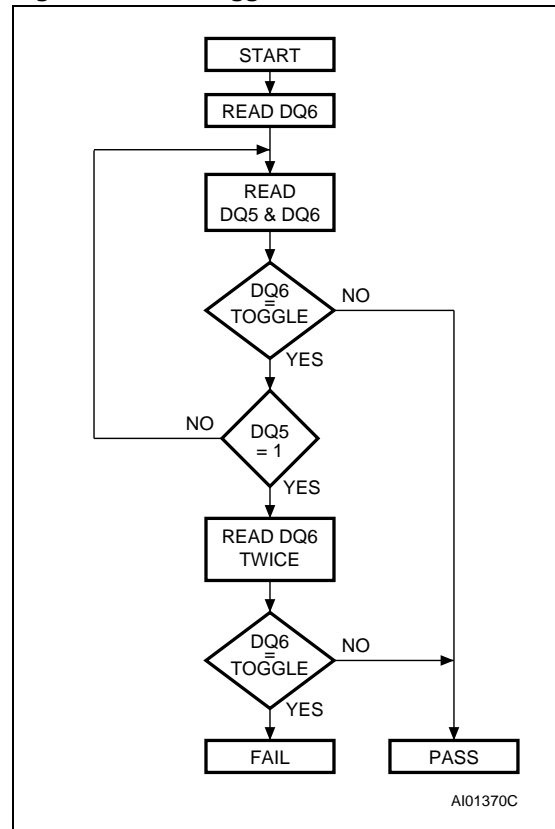
Figure 10. Data Toggle Flowchart
