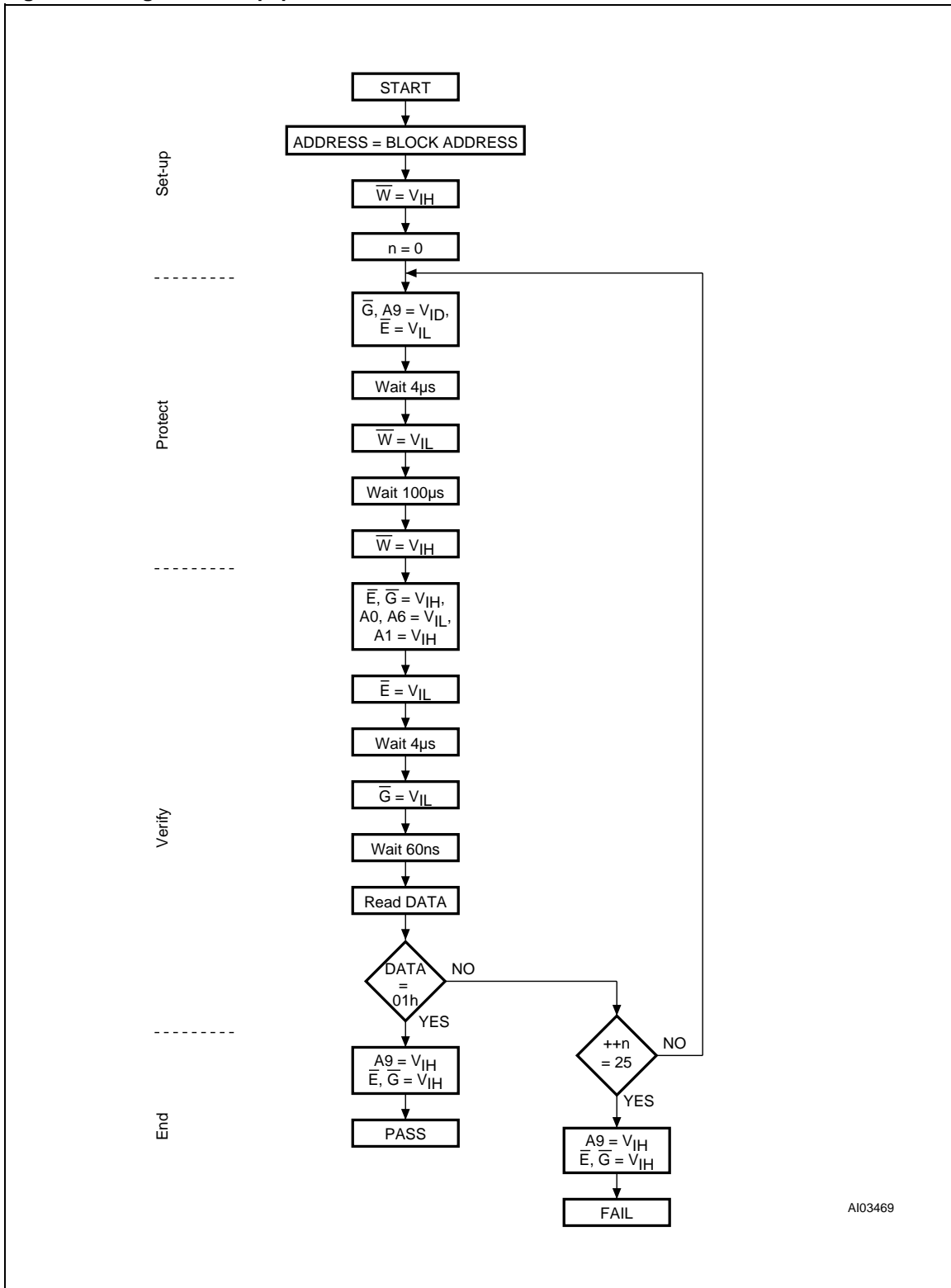
Figure 21. Programmer Equipment Block Protect Flowchart
