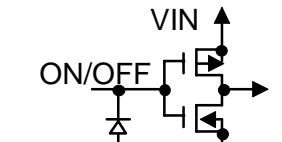
Figure 8 ON/OFF Pin
