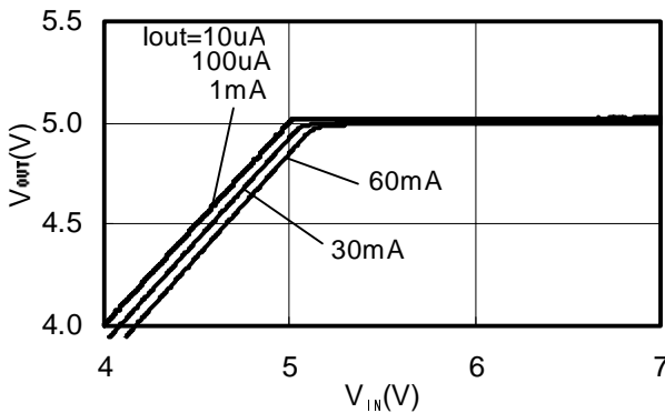
S-818A50A (Ta=25°C)
