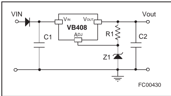
Figure 3: Start-up circuit
