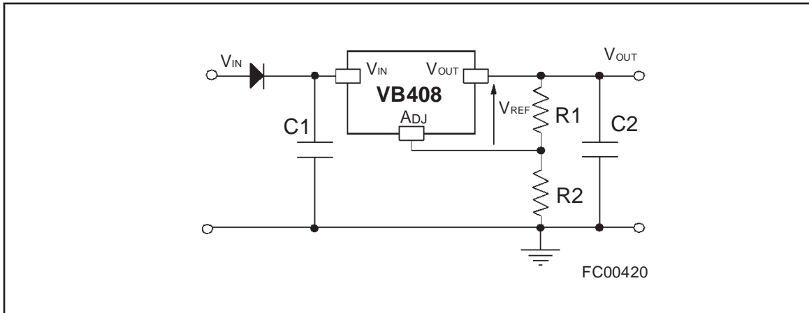
Figure 1: Typical application diagram
