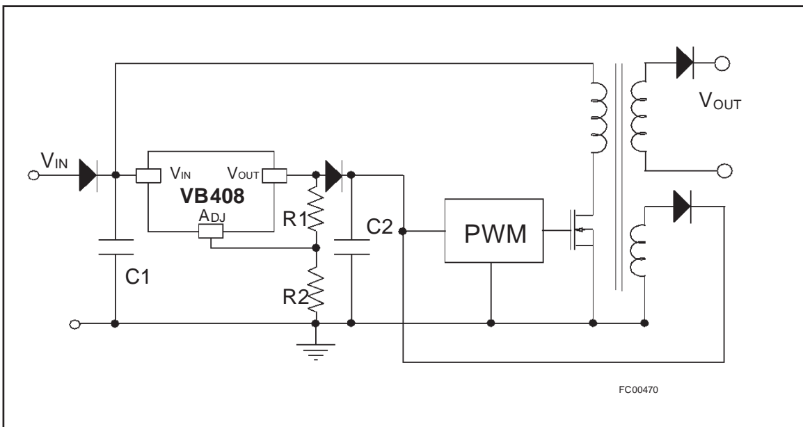
Figure 3: Start-up circuit
