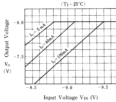
NJM79L08 Dropout Characteristics
