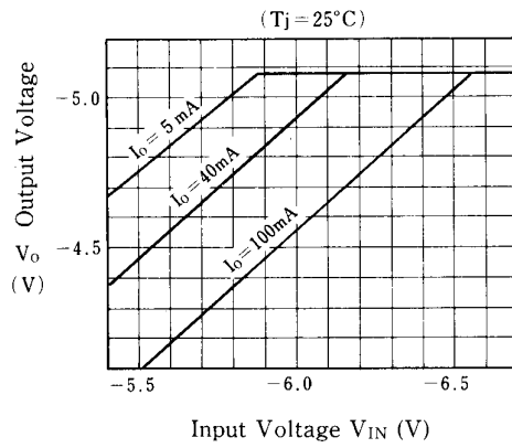
NJM79L05 Dropout Characteristics
