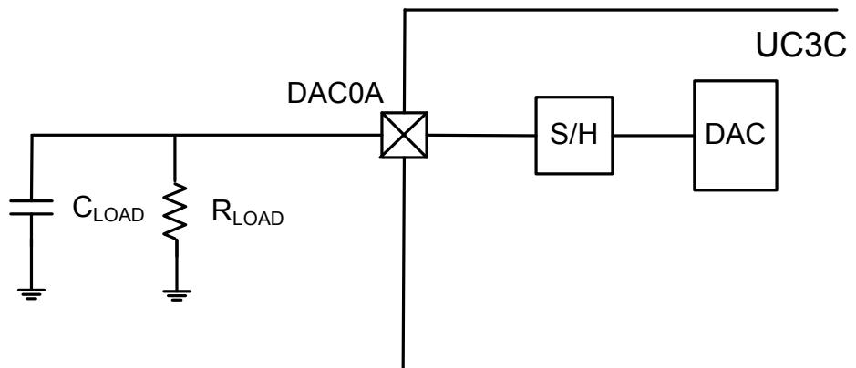
Figure 7-4. DAC output
