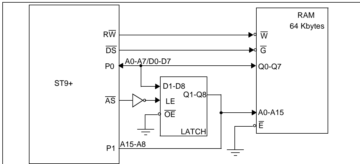
Figure 60. Application Example
