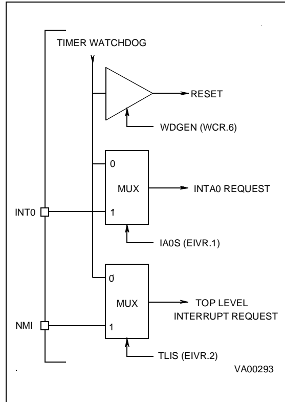
Figure 51. Interrupt Sources
