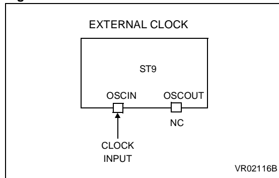
Figure 36. External Clock
