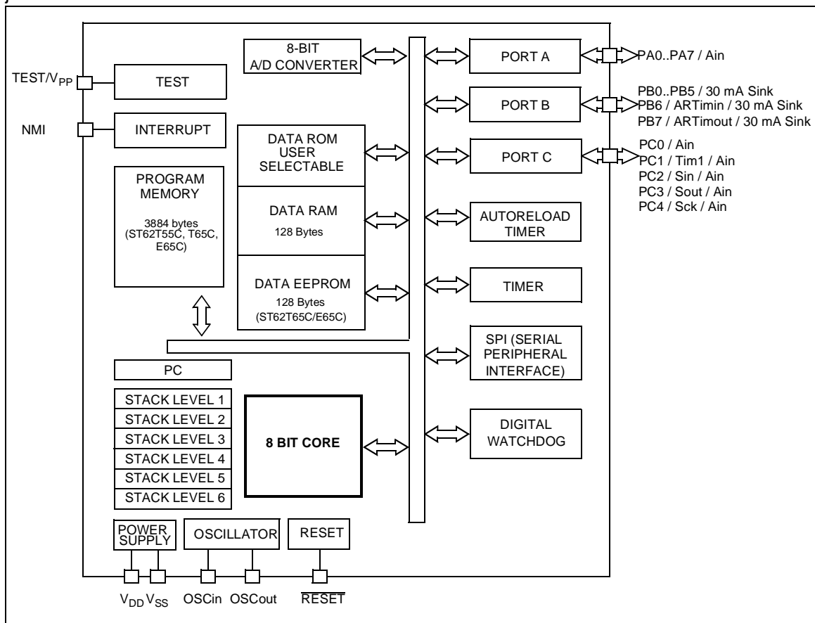
Figure 1. Block Diagram
