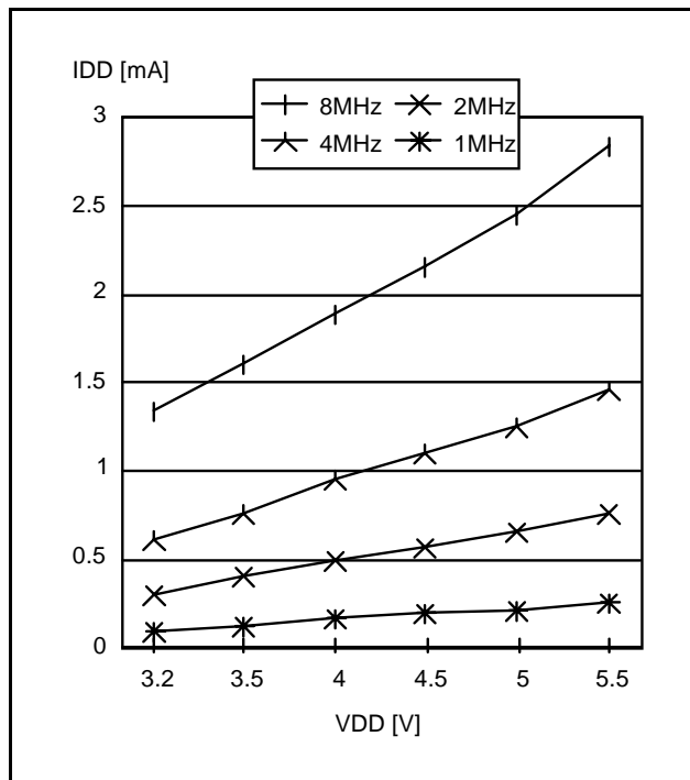
Figure 65. Typical I_{DD} in WAIT vs. f_{CPU}
