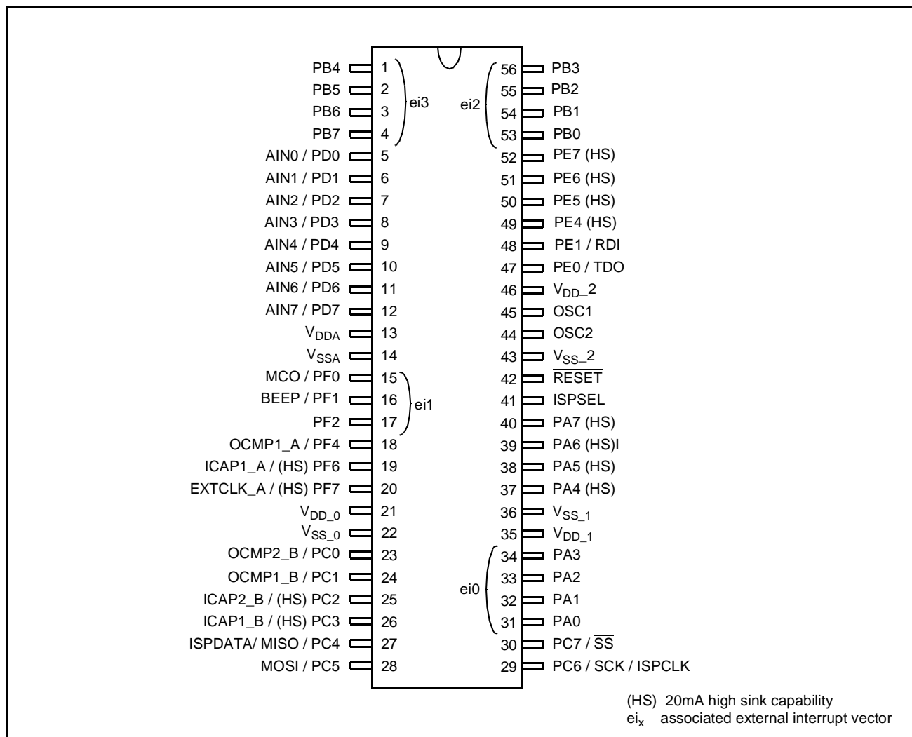
Figure 3. 56-Pin SDIP Package Pinout (N versions)
