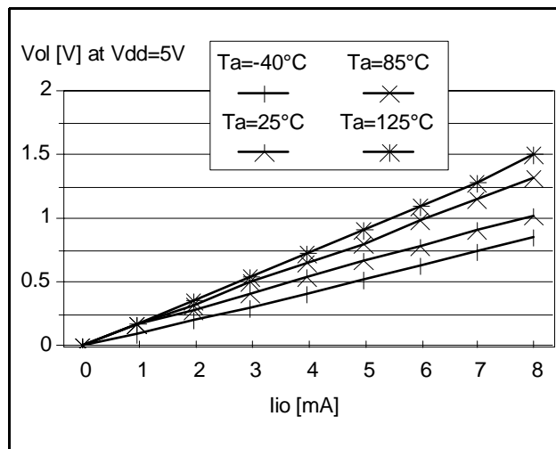
Figure 92. Typical V_{OL} at V_{DD}=5V ( \overline{RESET} )
